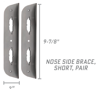
11002-75333: MOUNT VERTICALLY ON NOSE SIDE
