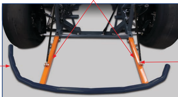
FRONT BUMPER MOUNTING KIT (HIGHLIGHTED IN ORANGE) WITH BLACK ADJUSTABLE BUMPER SUPPORTS
