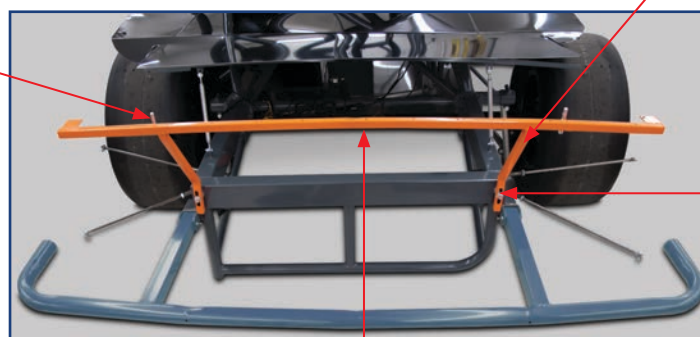
FULLY INSTALLED REAR DECK MOUNTING KIT (HIGHLIGHTED IN ORANGE)
